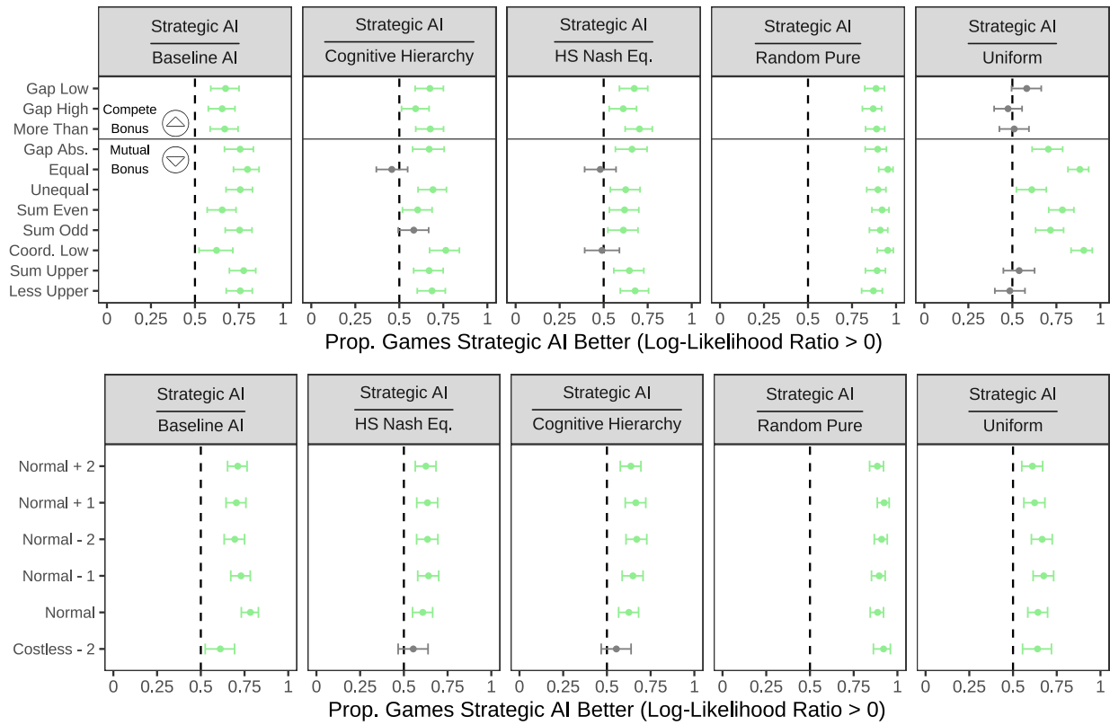
Figure D7: Relative predictive accuracy of the strategic AI agent vs other models for different game types ( \varepsilon = 0.2 )
