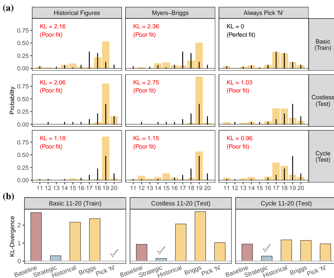
Figure 4: Response distributions for the 11-20 games with atheoretical AI agents
