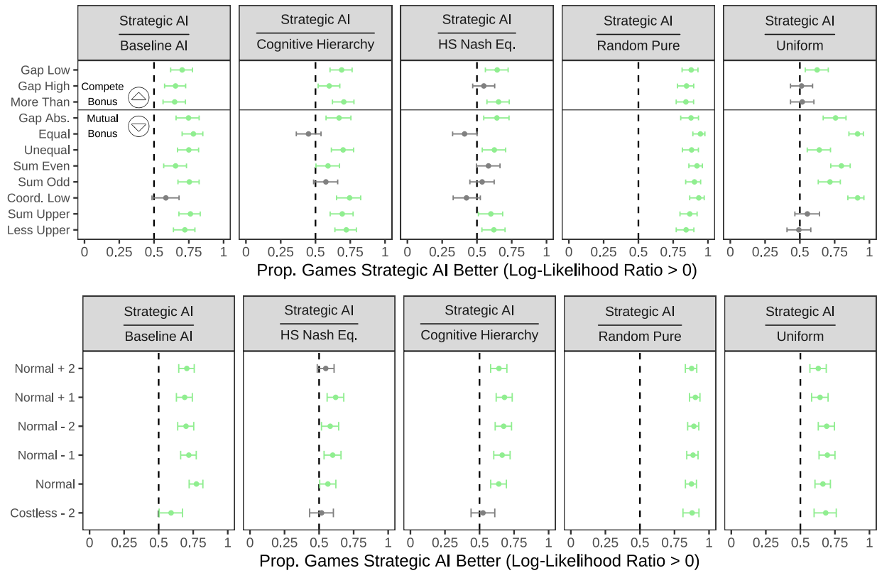
Figure D8: Relative predictive accuracy of the strategic AI agent vs other models for different game types ( \varepsilon = 0.3 )
