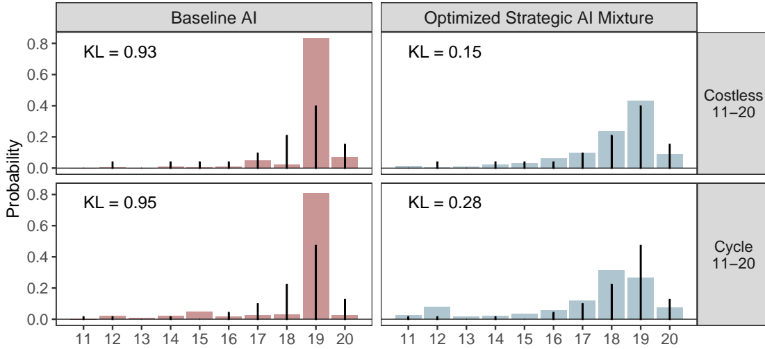
Figure 3: Response distributions for the cycle and costless versions of the 11-20 game
