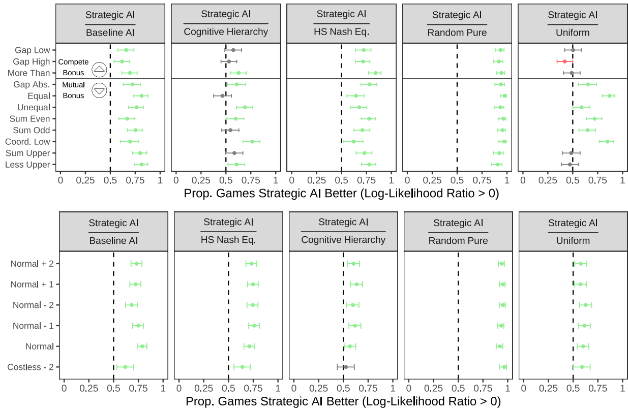
Figure D5: Relative predictive accuracy of the strategic AI agent vs other models for different game types ( \varepsilon = 0.05 )
