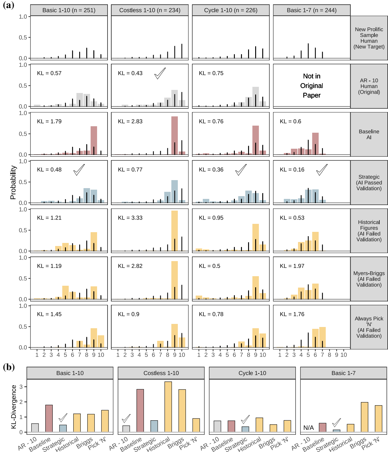
Figure 5: Analysis of novel 1-10 games: response distributions and KL divergences
