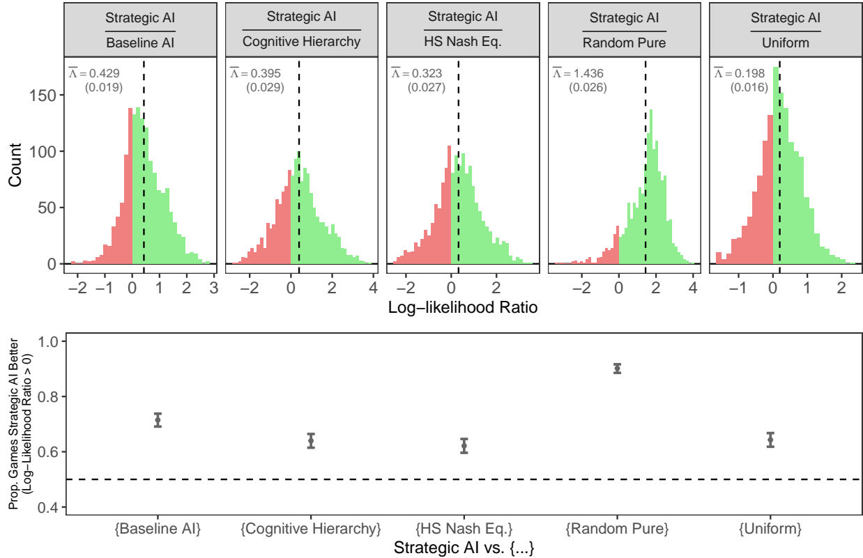
Figure 7: Predictive power of strategic AI agents compared to other models ( \varepsilon = 0.2 )
