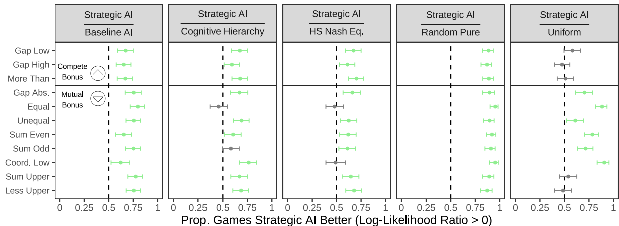
Figure 8: Relative predictive power of strategic AI agents ( \varepsilon = 0.2 ) by bonus rule
