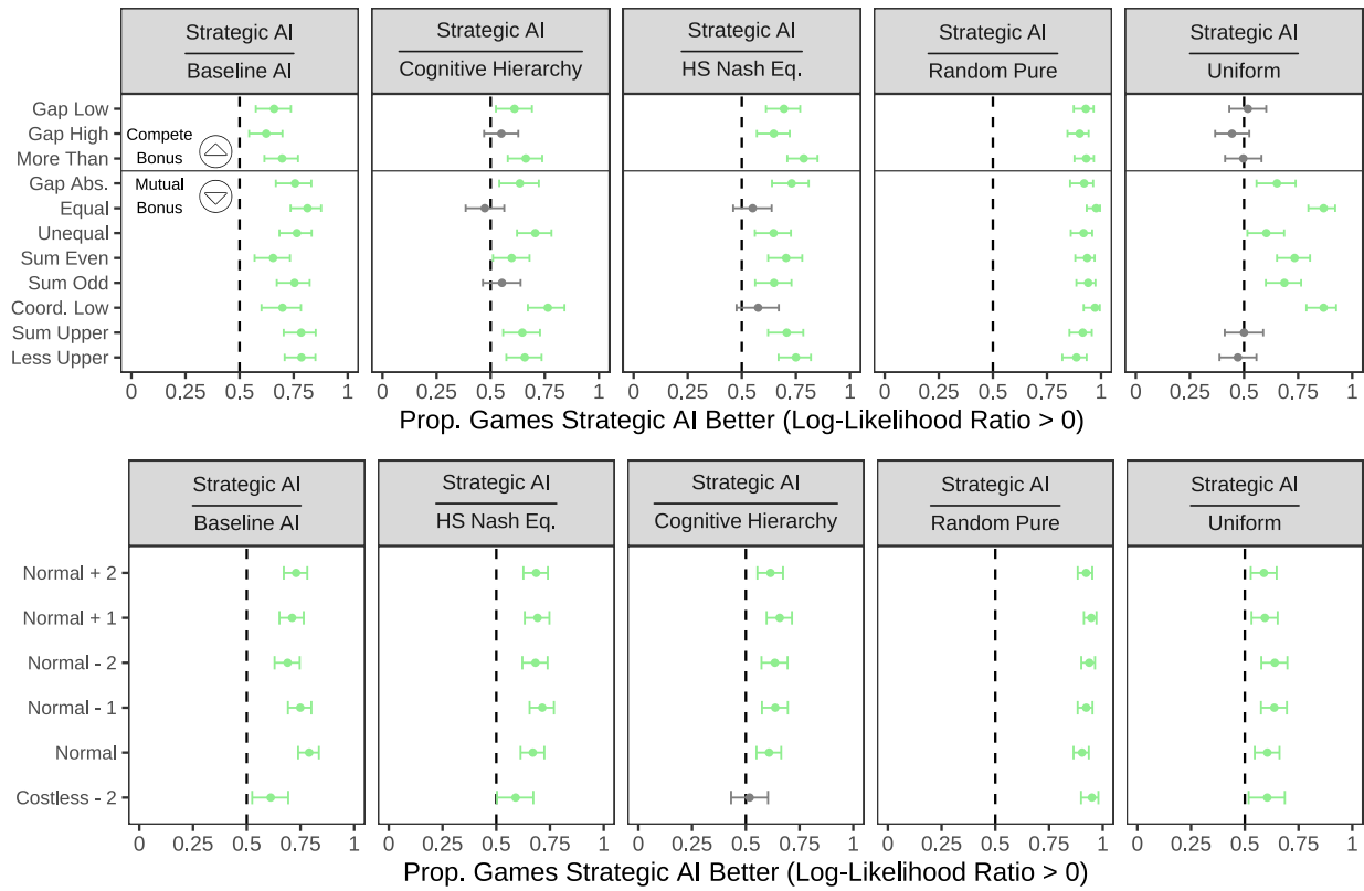
Figure D6: Relative predictive accuracy of the strategic AI agent vs other models for different game types ( \epsilon = 0.1 )
