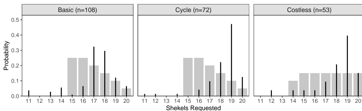
Figure 1: Nash equilibrium predictions and human responses in the 11-20 games
